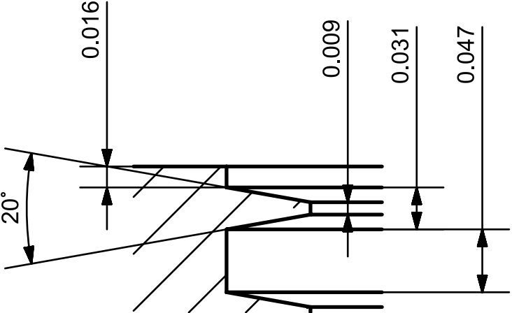
DETAIL B SCALE 10:1
